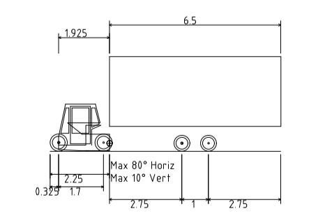
Electric Tug Side View:
