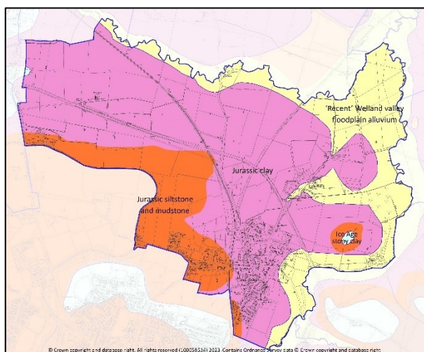
Figure 3.1: Geology of the Neighbourhood Area
