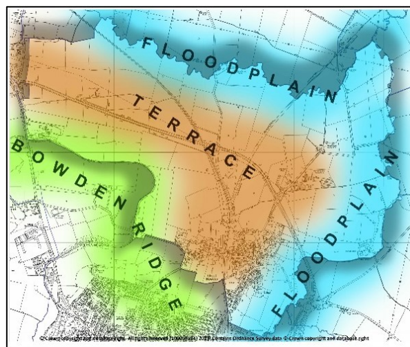
Figure 3.2: Topographic areas in the Neighbourhood Area, showing Great Bowden's position between the Bowden Ridge and the river floodplain
